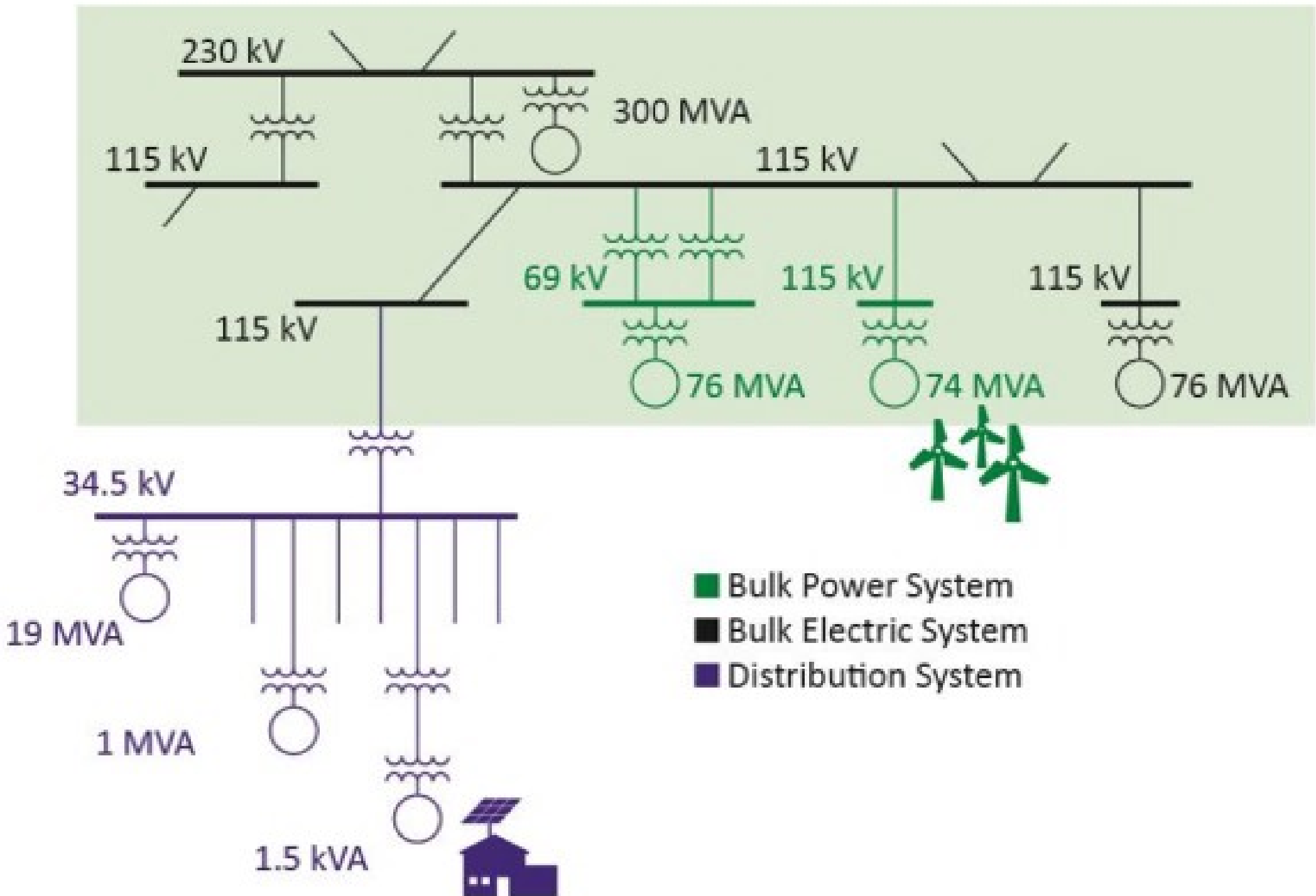
Figure 1: Designation of BPS, BES, and Distribution-Connected Resources
